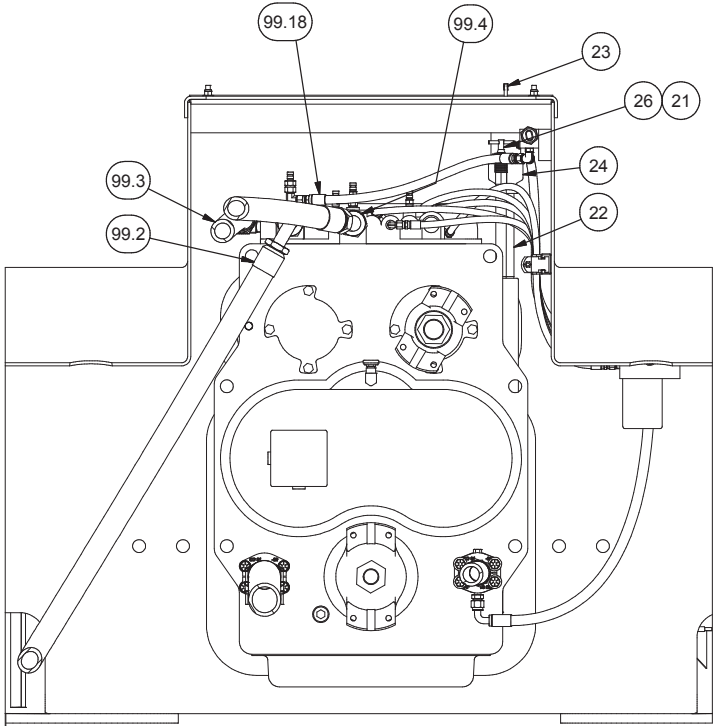
SECTION 4H-4H
