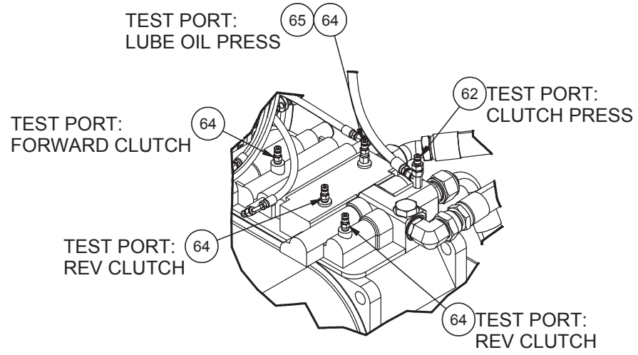
DETAIL 1A TEST PORT LOCATIONS
