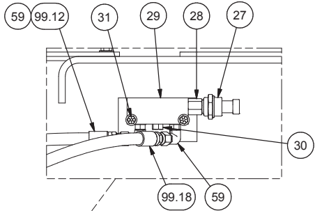
DETAIL 4M
